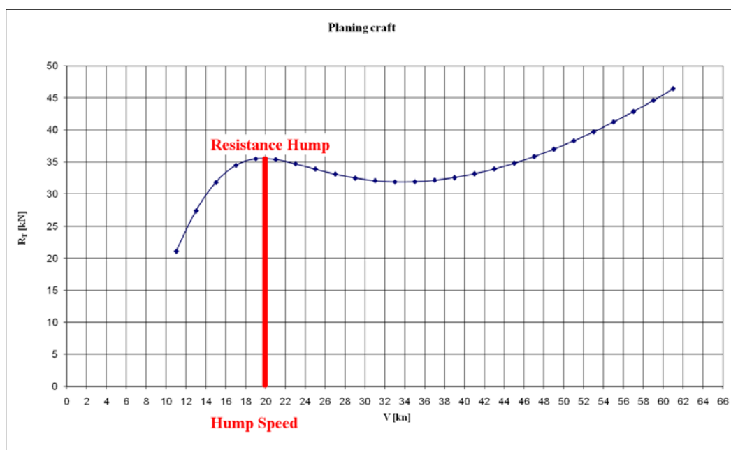
Figure 57: Resistance curve of a planing craft
