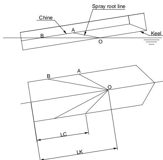
Figure.35: Characteristic lengths for a planing hull under way
