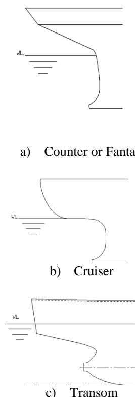
Figure 61: Types of stern profile
