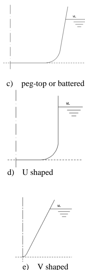
Figure 51: Typical shapes of transverse ship sections
