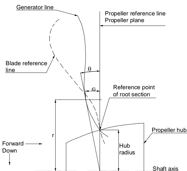
Figure 43: Diagram showing recommended reference lines (looking to port)
