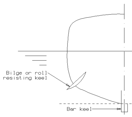
Figure 31: Bilge and bar keels
