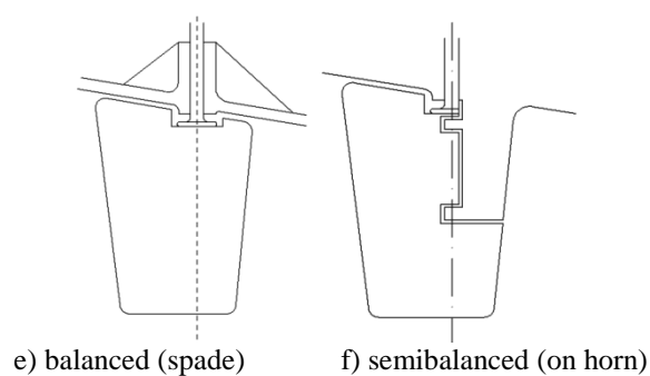
Figure 50: Rudder types
