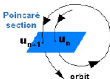
Figure 8: Poincare Map
