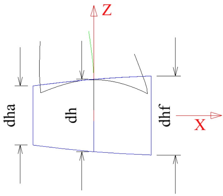
Figure 29: Hub diameters
