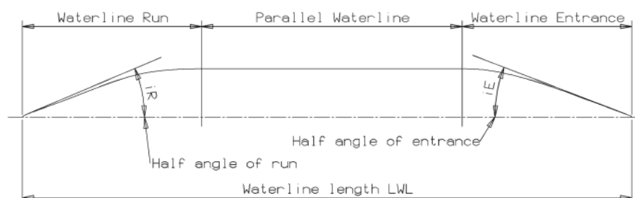
Figure 63: Waterline characteristics
