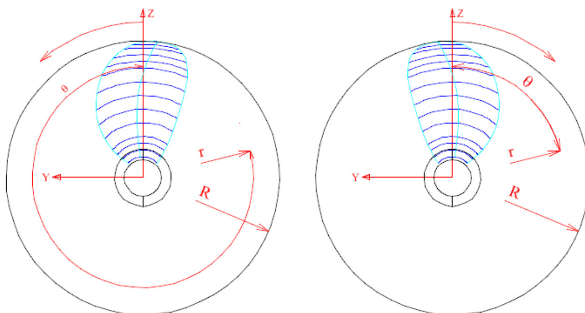
Figure 45: Propeller reference system, cylindrical, looking forward
