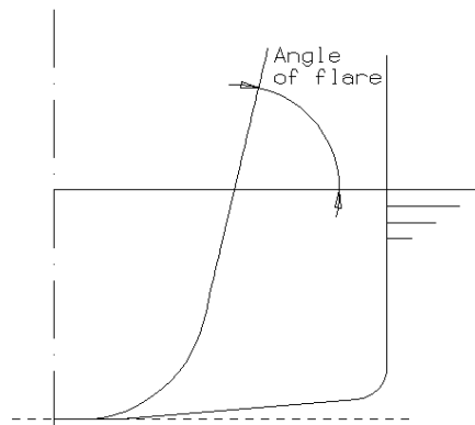
Figure 27: Transverse ship section with flare
