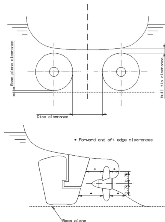
Figure 22: Propeller clearances
