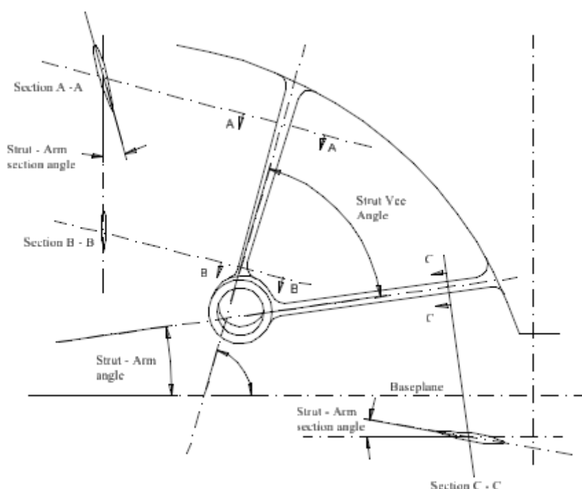
Figure 62: Characteristics of propeller strut or shaft bracket
