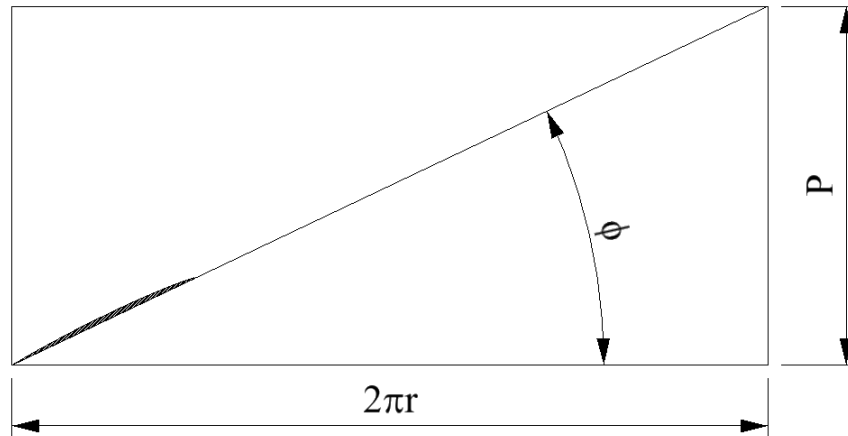
Figure 37: Pitch and Pitch Angle of a blade section
