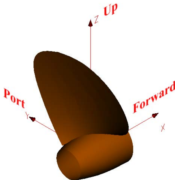
Figure 46: Propeller reference system, rectangular
