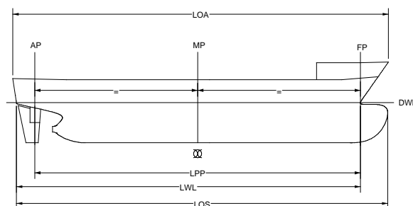
Figure 34: Characteristic ship lengths
