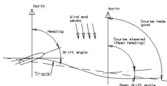
Figure 23: Course characteristics
