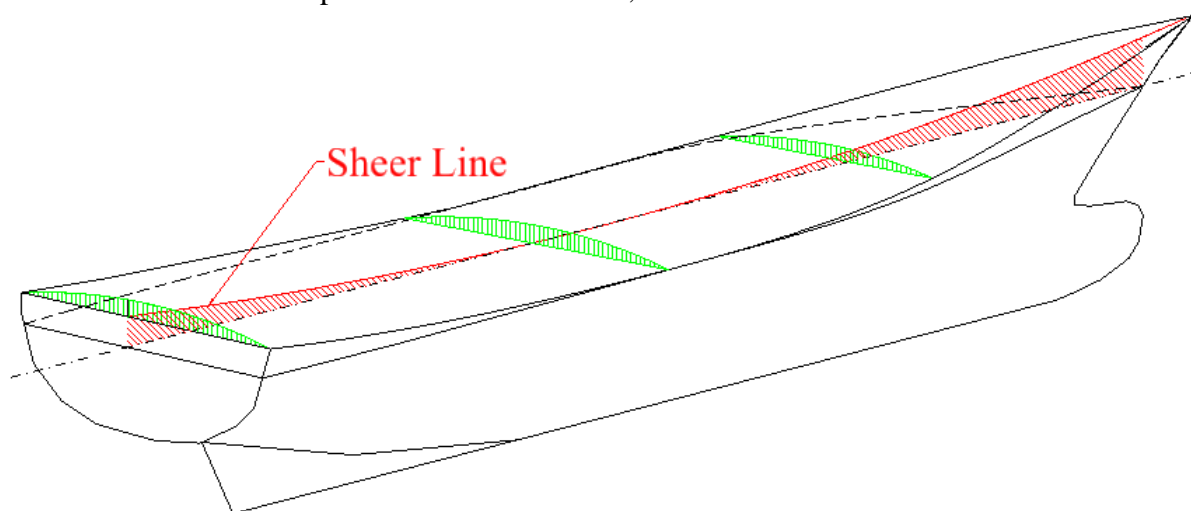
Figure 54: Definition of Sheer line
