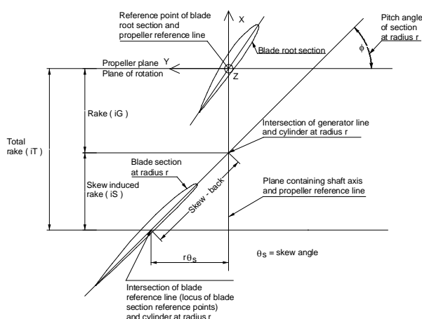
Figure 48: View of unrolled cylindrical sections at blade root and at any radius r of a right-handed propeller (looking down) showing recommended position of propeller plane.
