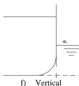
Figure 59: Types of stem profile
