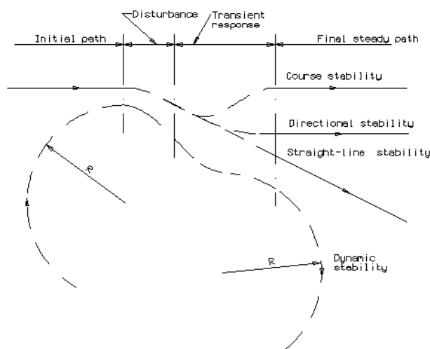
Figure 58: Illustration of stability items
