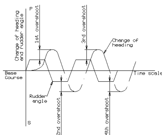
Figure 65: Zigzagging
