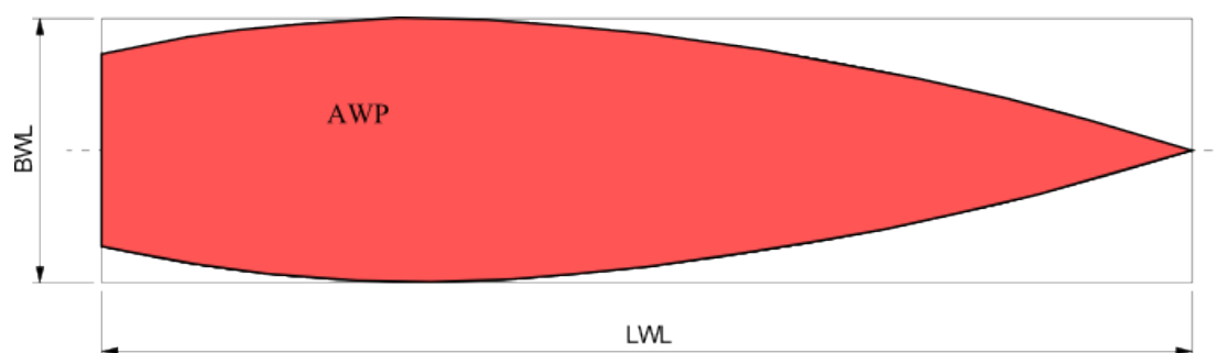
Figure 64: Waterplane area coefficient
