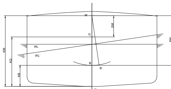
Figure 36: Transverse metacentric parameters
