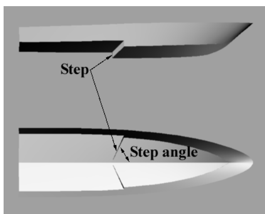
Figure 60: Step in planing craft hull
