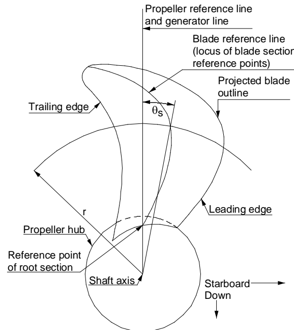
Figure 28: Diagram showing recommended reference lines (looking forward)
