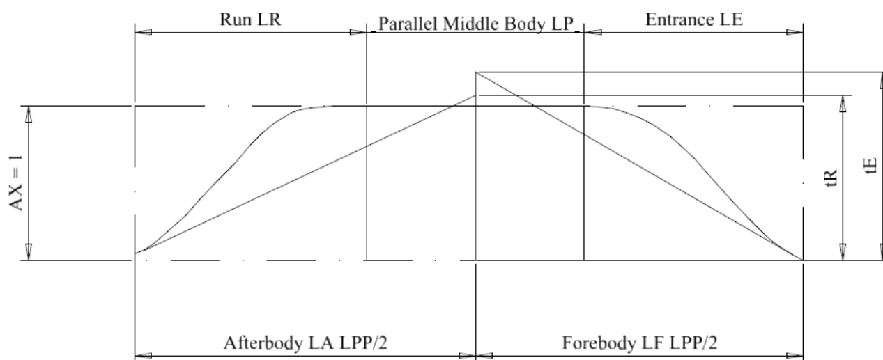
Figure 52: Characteristics of sectional area curve
