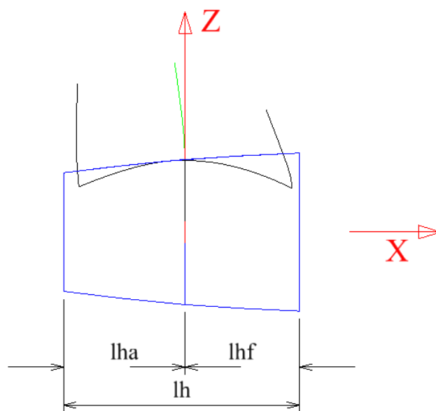
Figure 30: Hub length
