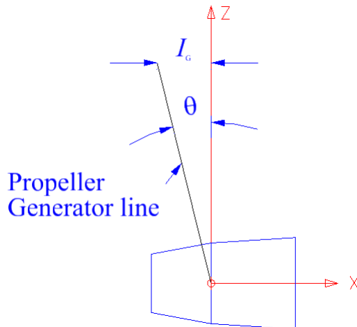
Figure 47: Definition of Rake at the blade tip and rake angle
