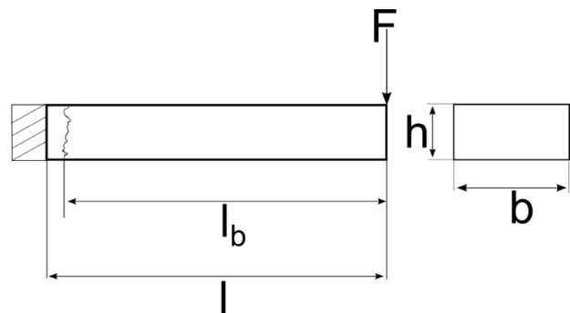
Figure 3: Beam dimensions
