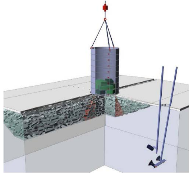
Figure 17 Circular cylinder with ballast weights is lowered down on the ridge
