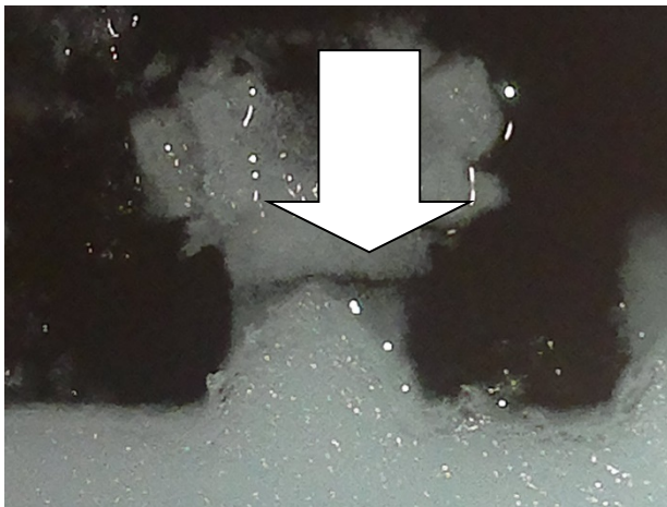
Figure 12: Compressive in-situ test with compressed cubic specimen and indicated loading direction
