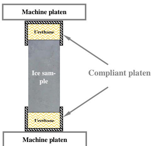
Figure 10: Compressive ex-situ test principle
