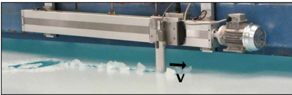
Figure 13: Measurement of crushing strength using the indenter test. A cylinder with a force sensor is pushed through the ice sheet with a constant velocity.
