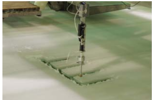
Figure 2: Setup of in-situ cantilever beam test
