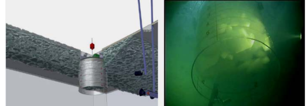
Figure 18 Illustration of macro-buoyancy cylinder penetrated through ridge (left), submerged translucent cylinder filled with ice-rubble (right)
