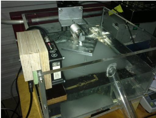
Figure 7: Ex-situ density measurement setup (Option B)
