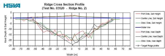
Figure 16 Cross section profiles of an ice ridge
