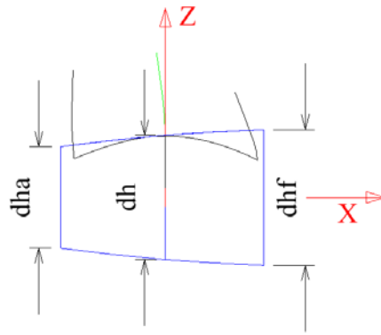
Figure 4-15: Hub diameters
