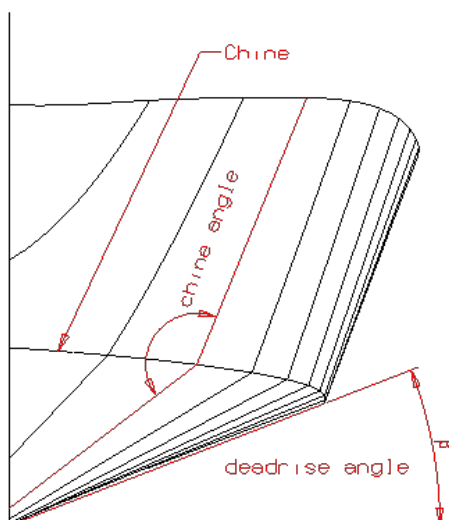
Figure 2-7: Hull form with chine
