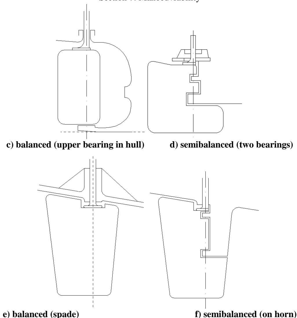
Figure 7-33: Rudder types.
