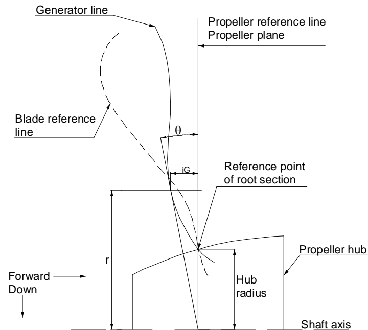
Figure 4-25: Diagram showing recommended reference lines (looking to port)
