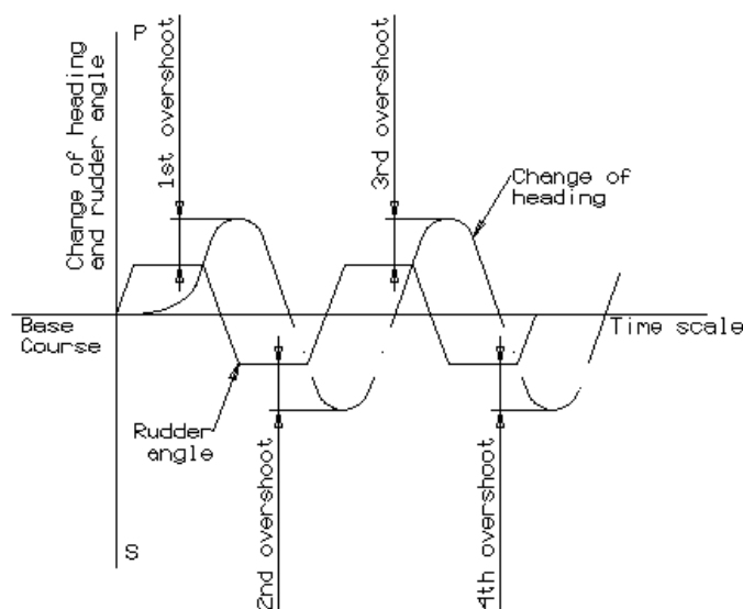
Figure 7-31: Zigzagging
