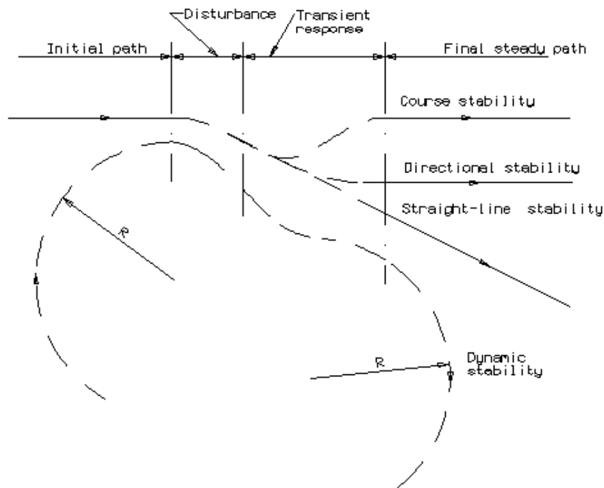
Figure 7-34: Illustration of stability items.
