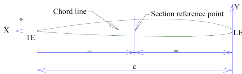
Figure 4-11: Unrolled generic propeller blade section
