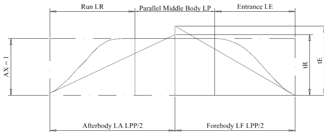
Figure 2-20: Characteristics of sectional area curve
