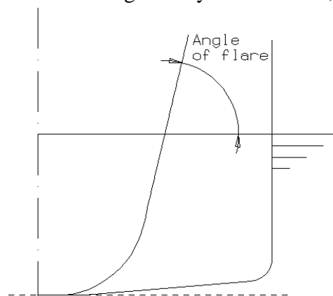
Figure 2-12 Transverse ship section with flare
