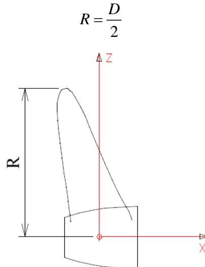
Figure 4-22: Propeller radius
