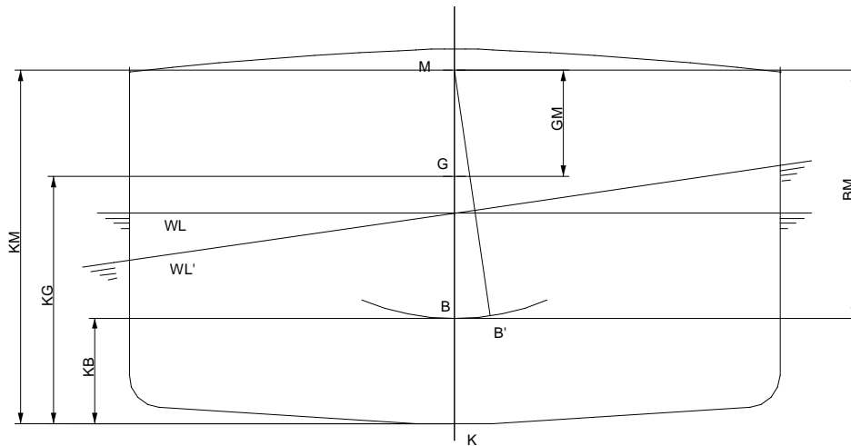
Figure 2-18 Transverse metacentric parameters
