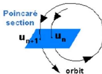
Figure 1-2 Poincaré Map
