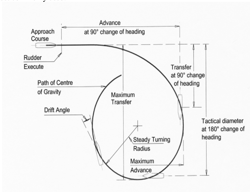
Figure 7-28: Geometry of turning circle
