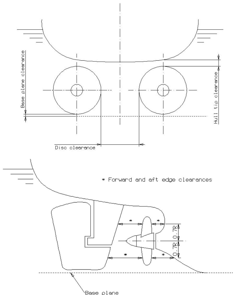
Figure 2-8: Propeller clearances
