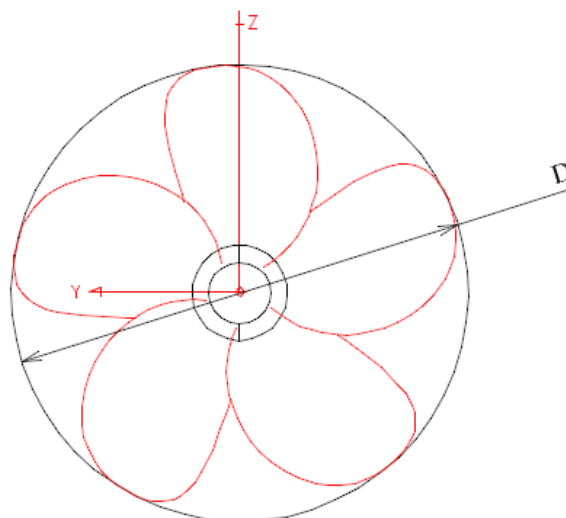
Figure 4-21: Propeller disk, looking forward
