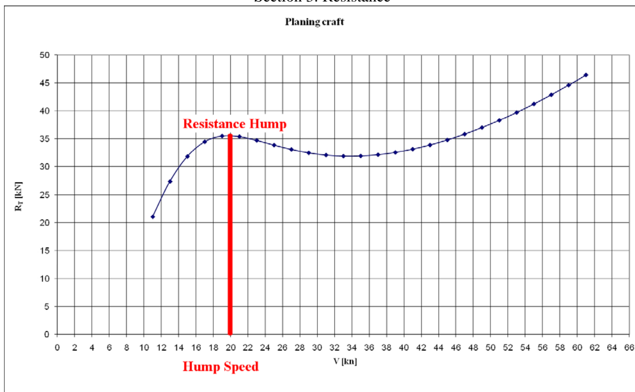
Figure 3-4: Resistance curve of a planing craft.
