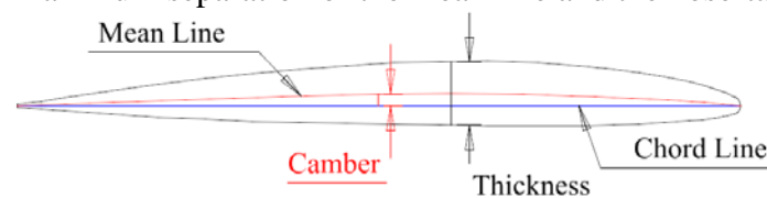
Figure 4-12: Blade section characteristics
