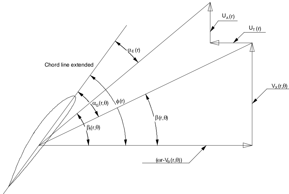
Figure 4-5: Typical velocity diagram for a propeller blade section at radius r
