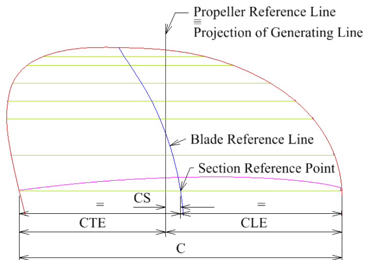
Figure 4-14: Portion of an expanded blade of a right handed propeller, showing Chord subdivision.
