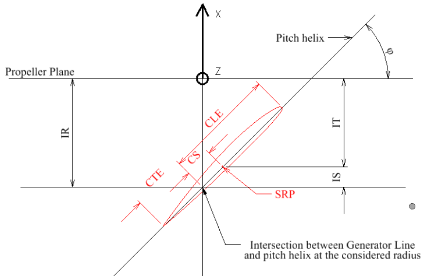
Figure 4-13: View of unrolled cylindrical section at radius r of a right-handed propeller (looking down) showing subdivisions of the Chord, Skewback and Rake.
