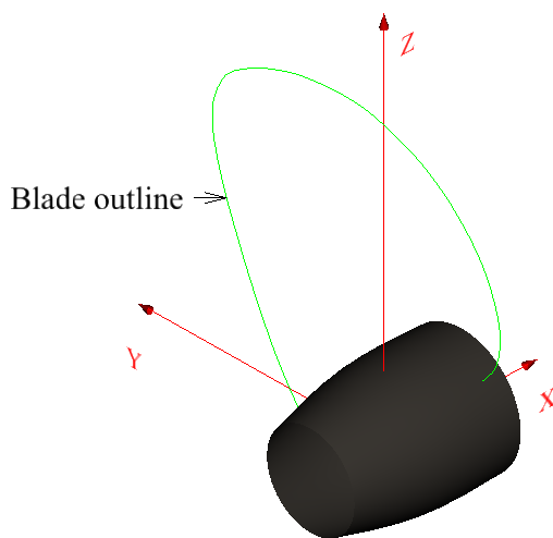
Figure 4-9: Propeller blade outline
