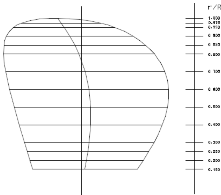
Figure 4-6: Expanded area of a propeller blade
