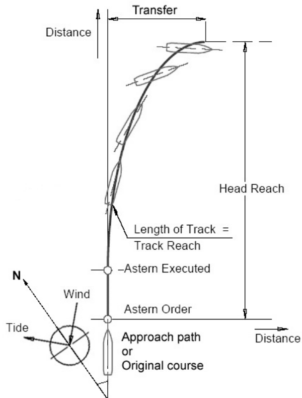
Figure 7-30: Crash back (stop) manoeuvre
