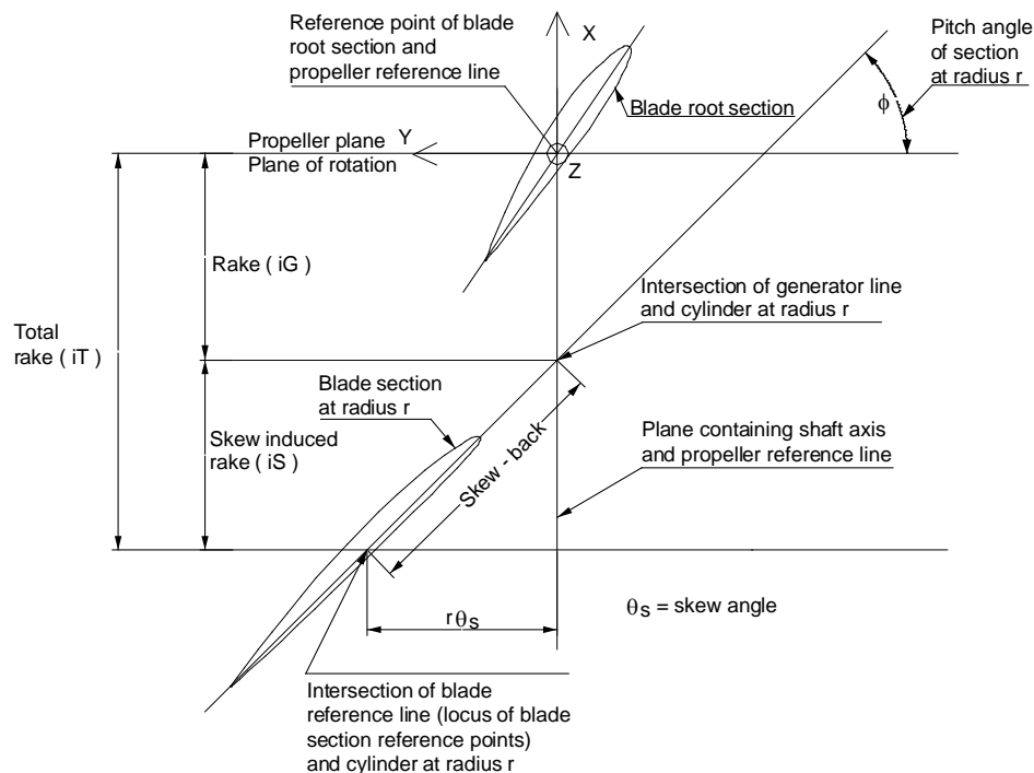
Figure 4-18: View of unrolled cylindrical sections at blade root and at any radius r of a right-handed propeller (looking down) showing recommended position of propeller plane.
