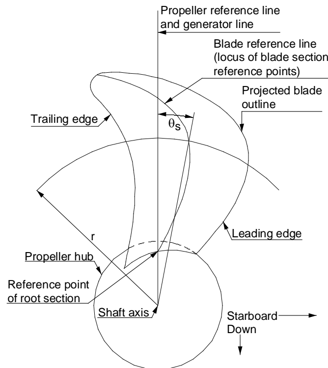
Figure 4-26: Diagram showing recommended reference lines (looking forward)
