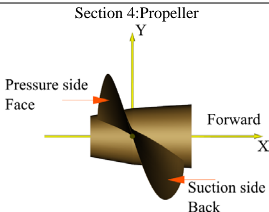
Figure 4-7: Propeller blade surfaces
