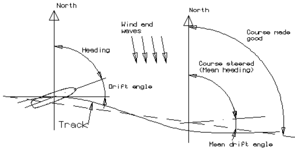
Figure 7-29: Course characteristics
