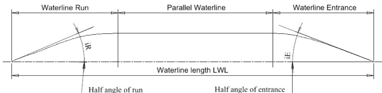
Figure 2-27: Waterline characteristics
