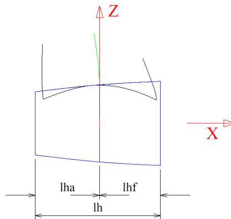
Figure 4-16: Hub length
