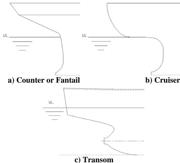
Figure 2-25 Types of stern profile
