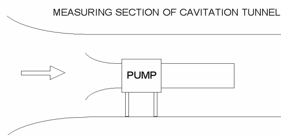
Figure 2.2 Installation of a pump model and bellmouth inlet within a cavitation tunnel
