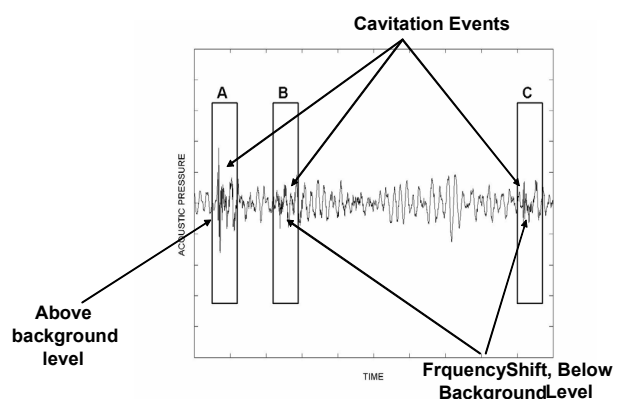
Figure 2.1 Measured SPL to determine acoustic cavitation inception
