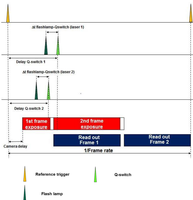
Figure 11. Timing diagram
