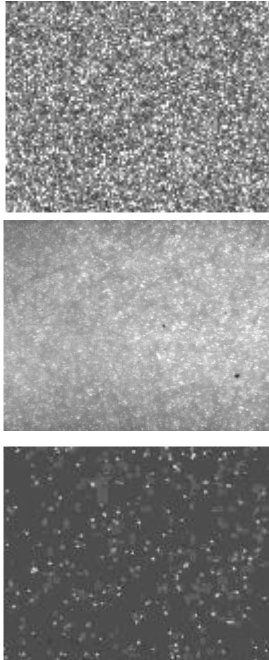
Figure 9. Example of a seeding distributions: suitable seeding distribution (top), defocused seeding distribution (mid), low seeding concentration (bottom)
