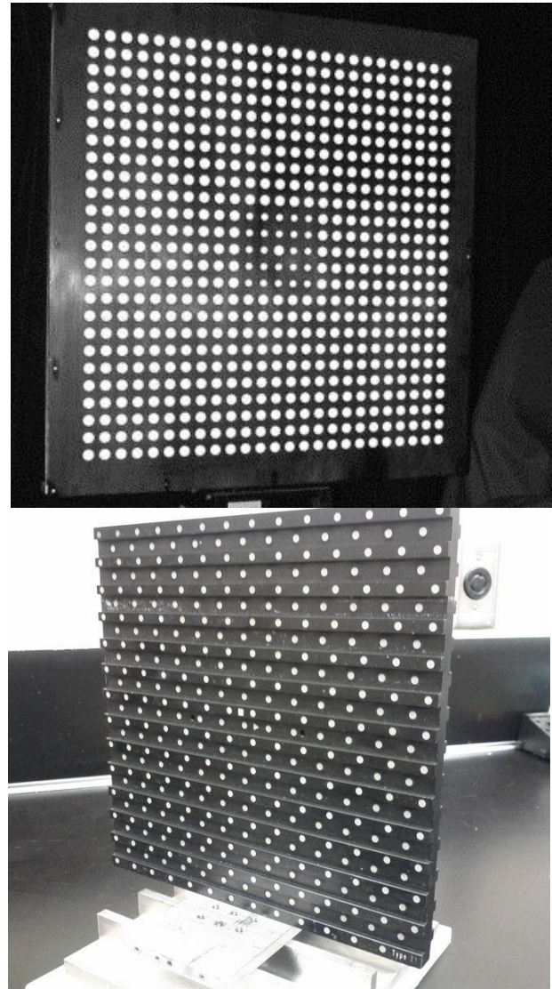
Figure 12. Calibration target for Stereo PIV: single-plane-double-side type (top), double-plane-double-side type (bottom)
