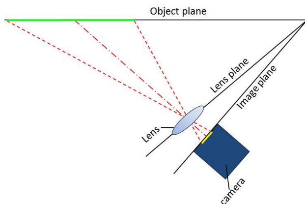
Figure 5. The Scheimpflug condition
