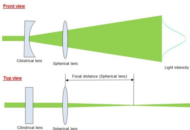
Figure 4. Light sheet generation
