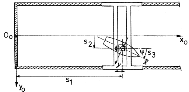
Figure 6: Computerized PMM with three degrees of freedom (position controlled).
