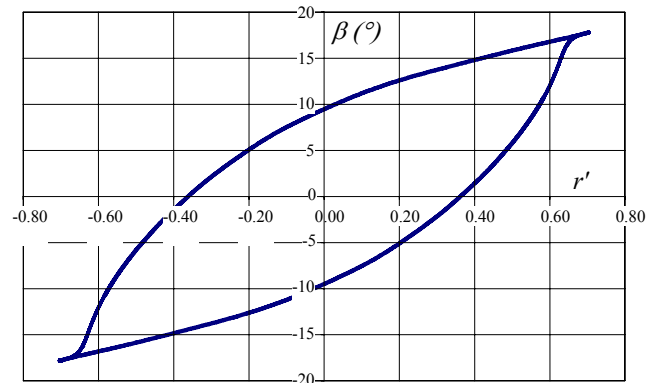
Figure 4: Yaw rate, drift angle envelope for a surface ship
