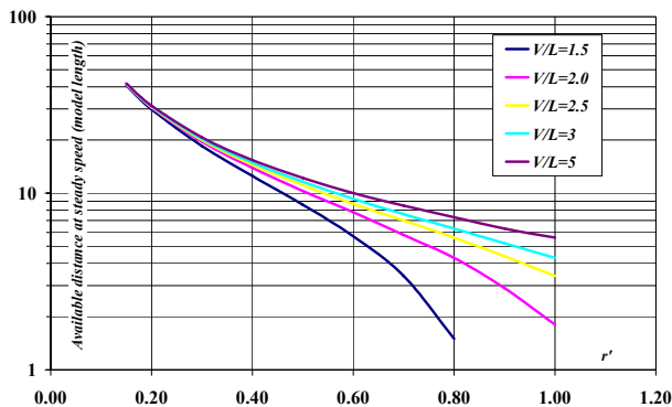
Figure 5: Influence of speed and r' on duration of stationary conditions (ship length) for a complete turn
