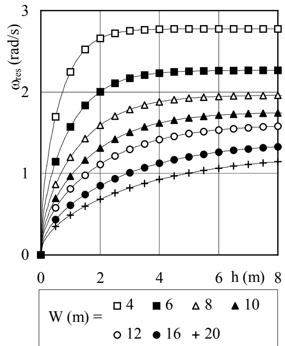
Figure 2: Lowest tank resonance frequency as a function of water depth h for several tank width values b .
