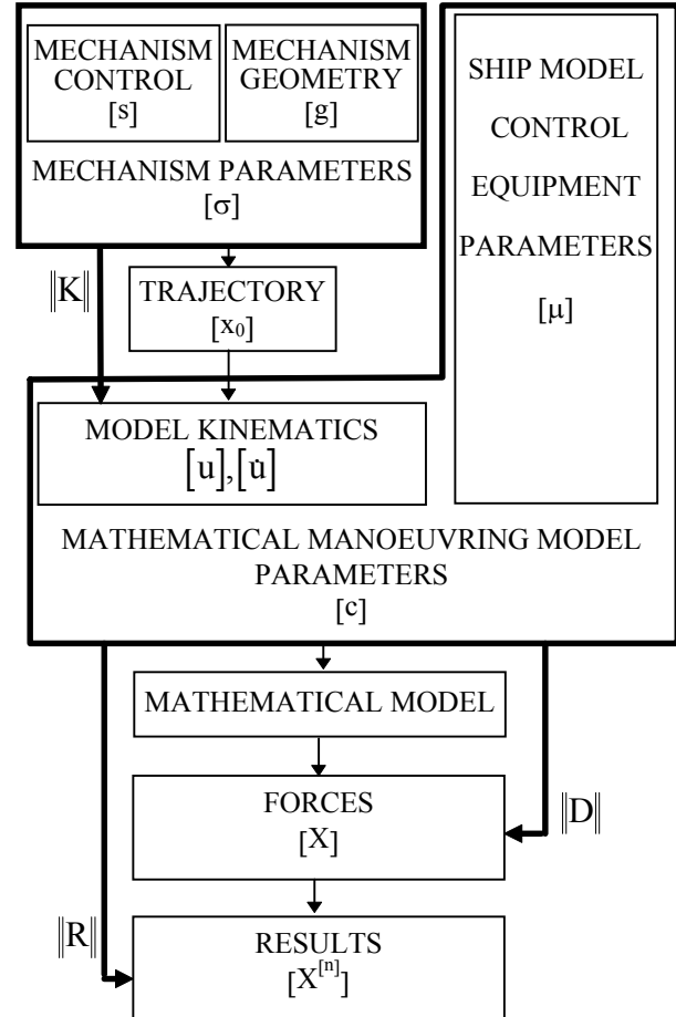
Figure 9: Overview of factors influencing accuracy of test results.
