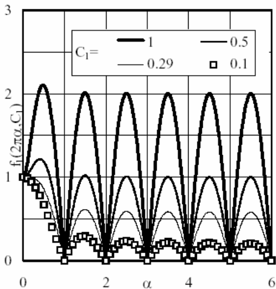
Figure 10. Function f_1(2\pi\alpha, C_1) for different C_1
