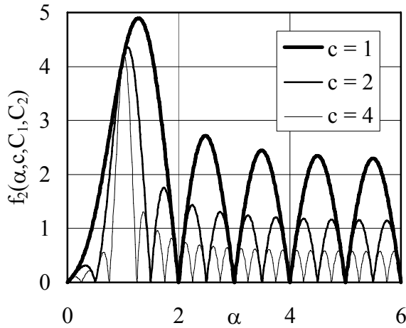
Figure 12: f_2 as a function of \alpha for different number of oscillation cycles ( C_1 = 0.552 ; C_2 = 3.52 - Esso Osaka , h/T = \infty , \omega'_1 = 5.23 ).
