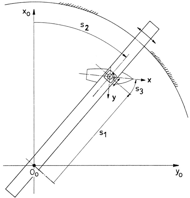
Figure 8: Rotating arm
