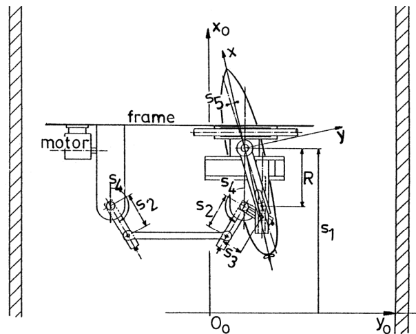
Figure 7: Large Amplitude PMM System (DMI type).
