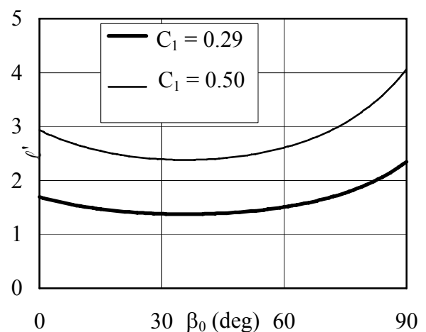
Figure 11: Esso Osaka ( h/T = 8 ): required measuring length for obtaining specified C_1 .
