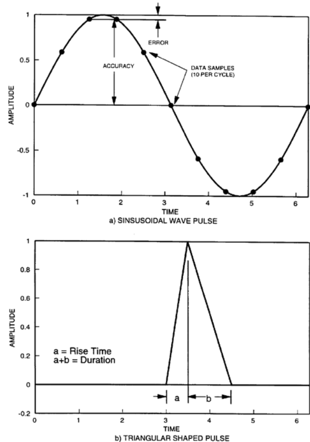
Figure 7. Examples of Loading Time Histories as Relates to Required Sample Rates (Dinsenbacher, 2010).
