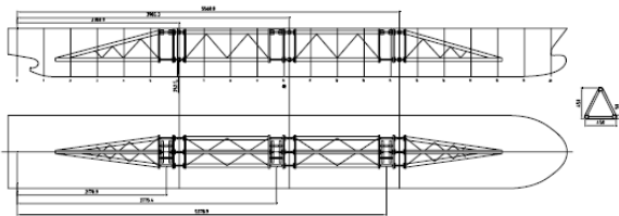
Figure 1. Elastic Segmented Model with Internal Backspine Beam (Miyake, 2009).
