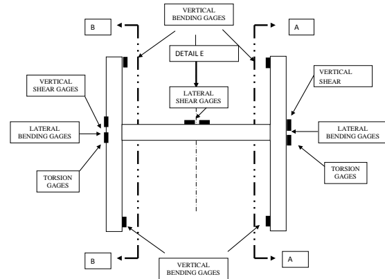
Figure 3. Possible Strain Gage Measurement for Internal Elastic Strength Bar (Dinsbacher, 2010).
