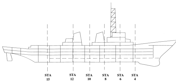
Figure 5. Example Segmentation Spacing (Dinsenbacher, 2010).
