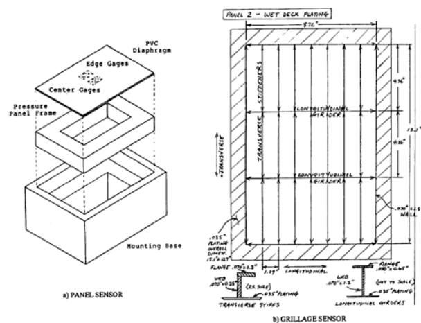
Figure 8. Example of Panel and Grillage Sensors (Dinsenbacher, 2010).
