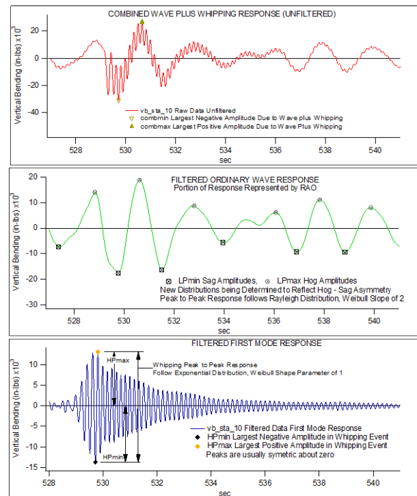
Figure 9. Example of Analysis to Filter and Arrive at First Mode and Whipping Responses (Dinsenbacher, 2010).
