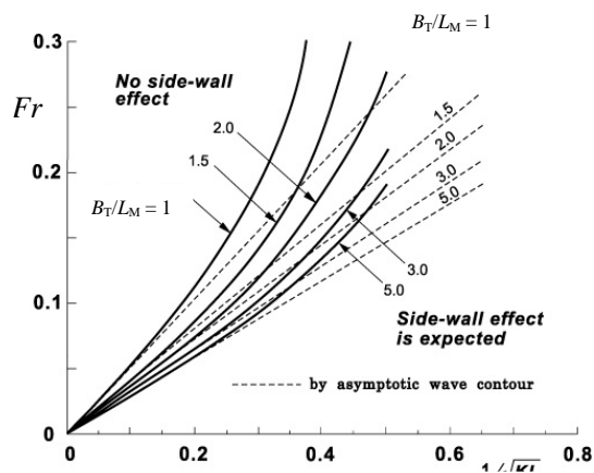
Figure 2. Estimation of tank-wall effects using unified slender theory (Kashiwagi & Ohkusu 1991).
