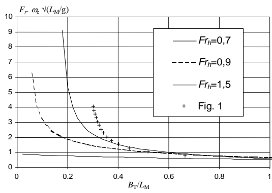
Figure 3. Maximum frequency at which tank interference occurs in head waves and finite depth.
