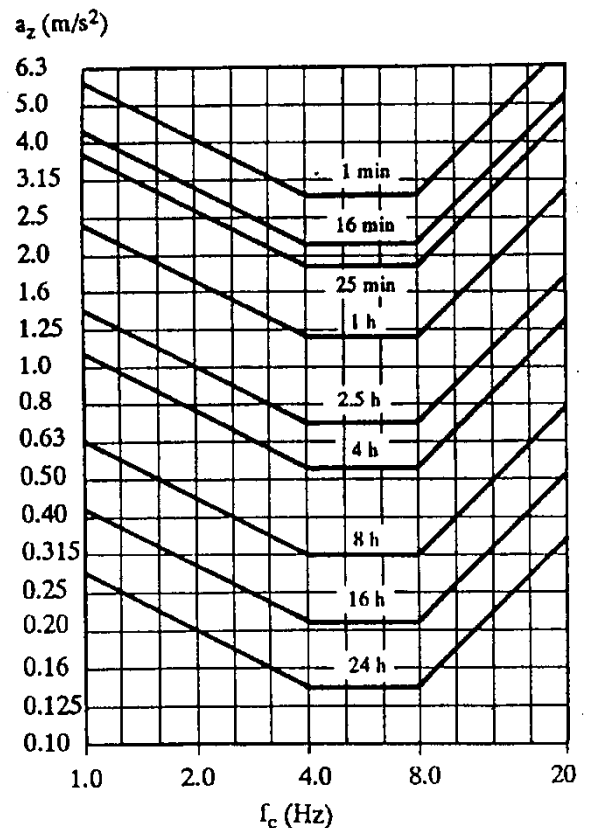
Fig. 2. ISO 2631/1 Fatigue-Decreased Proficiency Boundaries
