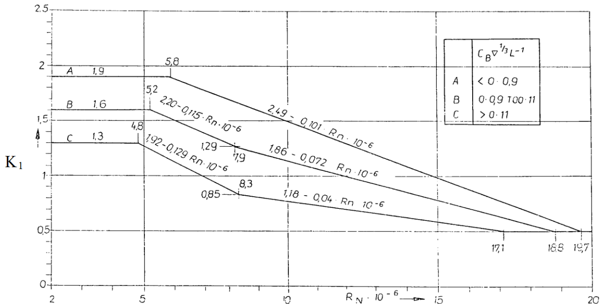
Fig. 4. Correction - factor K_1 (Scott [2.16])
